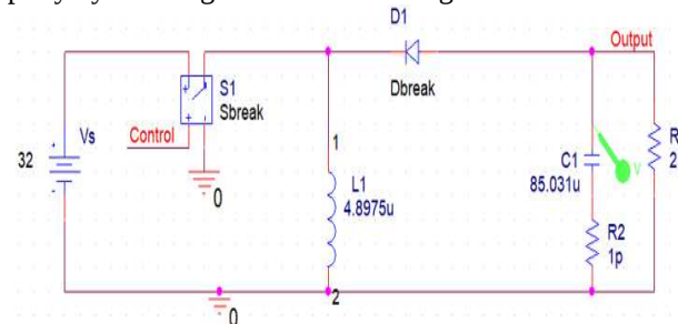
Figure 7: Buck-Boost Converter Schematic Diagram
