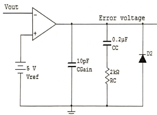
Figure 13: Error Amplifier Circuit
