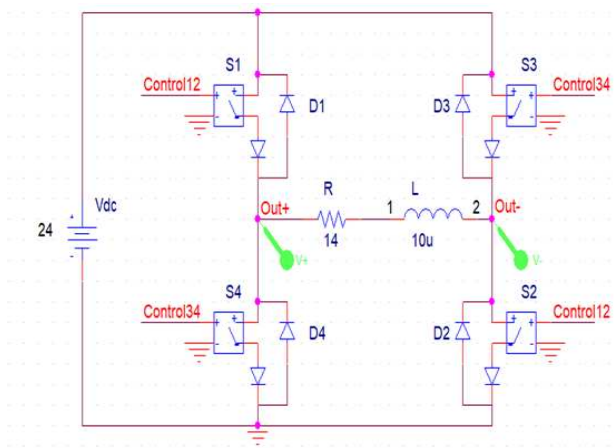
Figure 9: Full H-Bridge Square Wave Inverter Schematic
