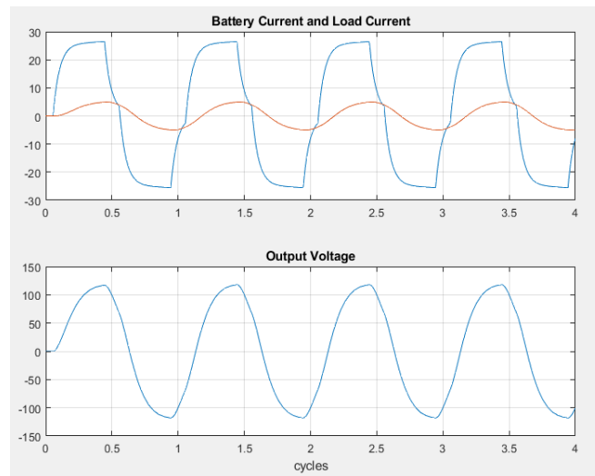
Figure12: Matlab Simulation Results for a Square wave inverter Circuit with Transformer and Capacitor
