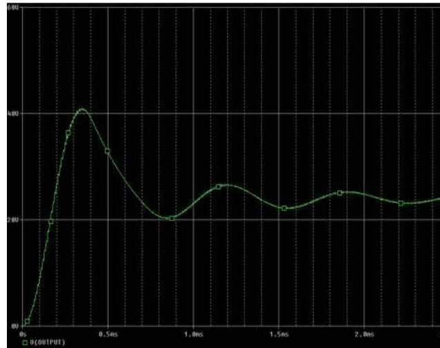
Figure 3: Output Voltage of Flyback Converter
