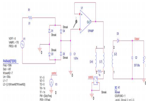
Figure 3: AC to DC Schematic Circuit in PSPICE
