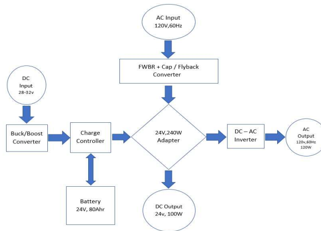
Figure 1: Universal Power Supply Adapter Block Diagram
