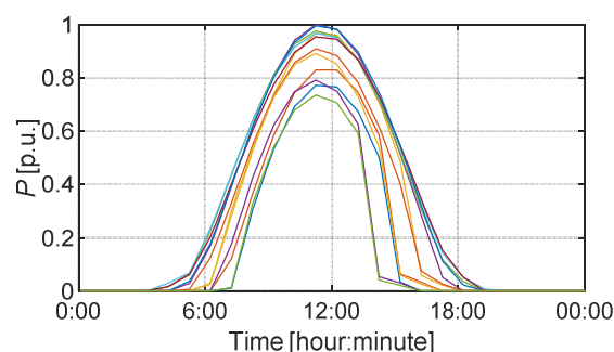
Fig.7. Normalised time-dependent output active power profile of a unity PV system for characteristic day in each month
