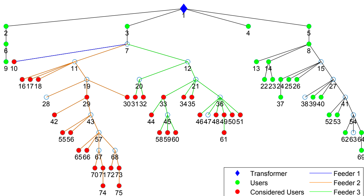
Fig. 2. Tree diagram of the discussed low-voltage grid
