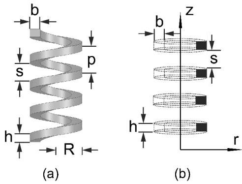
Fig. 1. (a) Schematic of the Air-Core Reactor Dimensions and (b) Representation of a Solid in an Axisymmetric Coordinate System.
