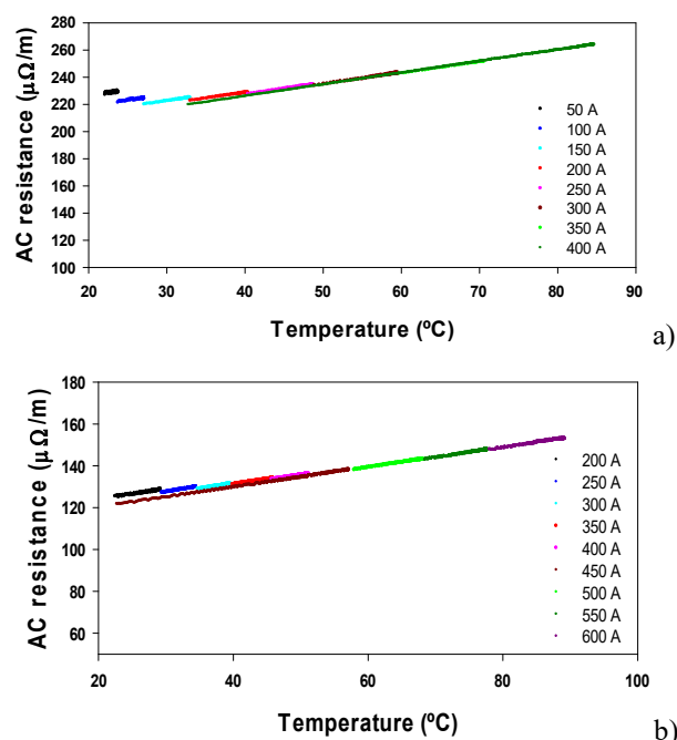
Fig. 9. Temperature and current dependency of the AC resistance. a) ACSR 135AL1 two-layer ACSR conductor. b) Crocus288 two-layer ACSR conductor.
