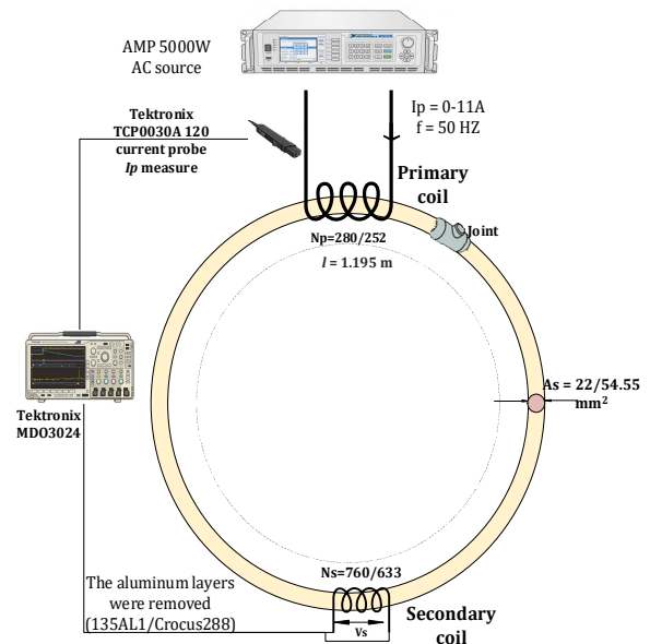
Fig. 2. Experimental setup used to determine the B and H fields as well as \delta_{eff} , \mu_{r,eff} and \mu_{r,eff}' . This setup was used to characterize the core of the Crocus 288 and 135AL1 conductors.
