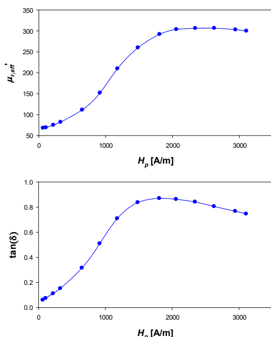
Fig. 8. Crocus288 conductor (double layer). Experimental values of \tan(\delta_{eff}) and \mu_{r,eff'} versus H_p at 59°C.
