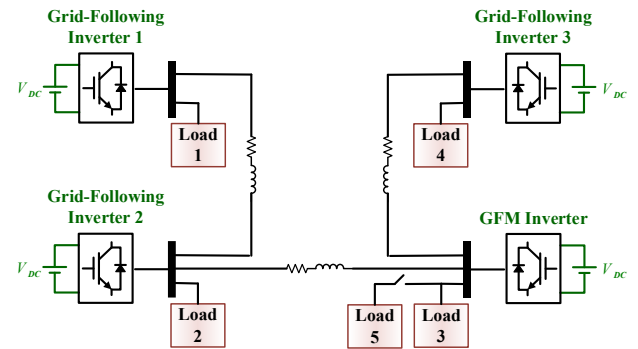
Fig. 3. Schematic diagram of the islanded microgrid under study [15].
