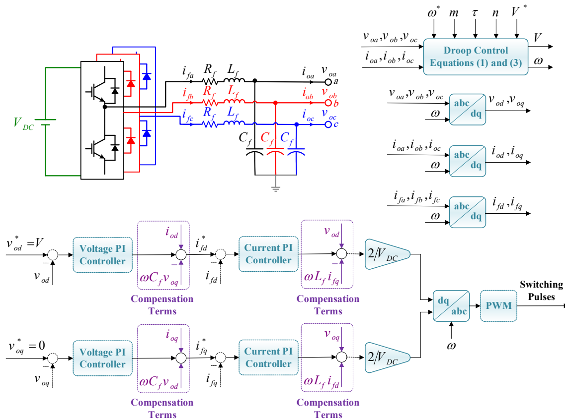
Fig. 1. Schematic diagram of droop control-based GFM inverter.
