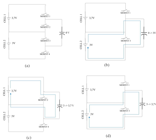
Fig. 3. Balancing operating sequence.
