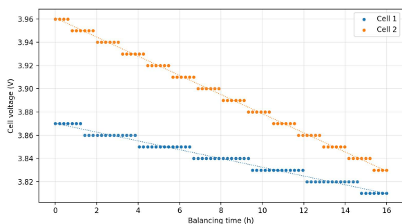
Fig. 7. Cell voltage evolution during active balancing
