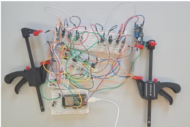
Fig. 5. Experimental setup.
