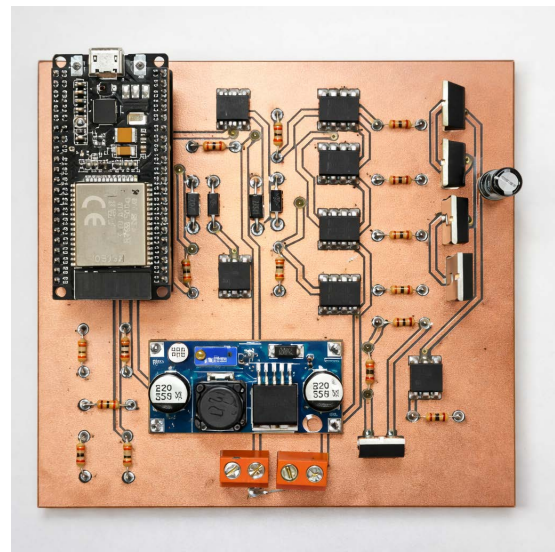
Fig. 6. Final PCB with components implemented.
