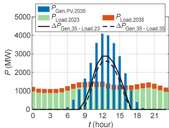
Fig. 7. The day with the highest positive hourly difference between PV generation and consumption power (29.4.2023)
