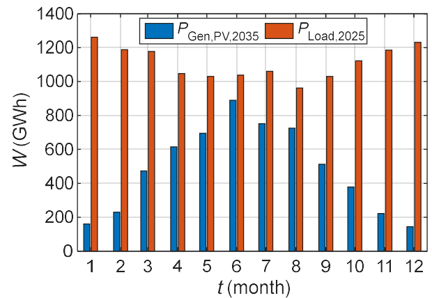
Fig. 6. Monthly energy profiles considering PV generation with installed PV power in 2035 and consumption in 2025
