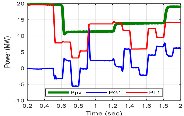
Fig. 8. Power response (Area 1).
