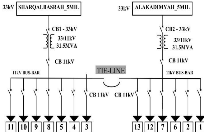
Fig. 3. The 33/11kV Substation of 5-mile proposed network simulated using CYME
