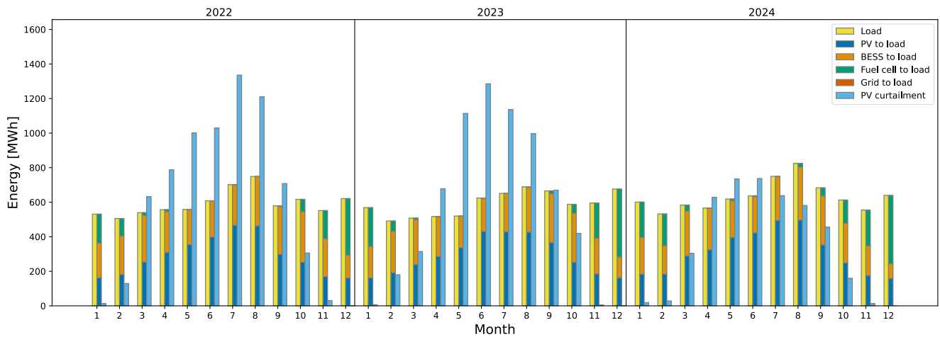
Fig. 6. Monthly load, supply allocation, and PV curtailment for hybrid BESS-Hydrogen configuration
