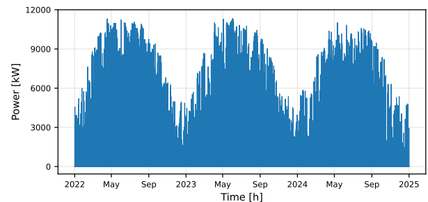
Fig. 3. Hourly PV generation profiles (2022–2024).
