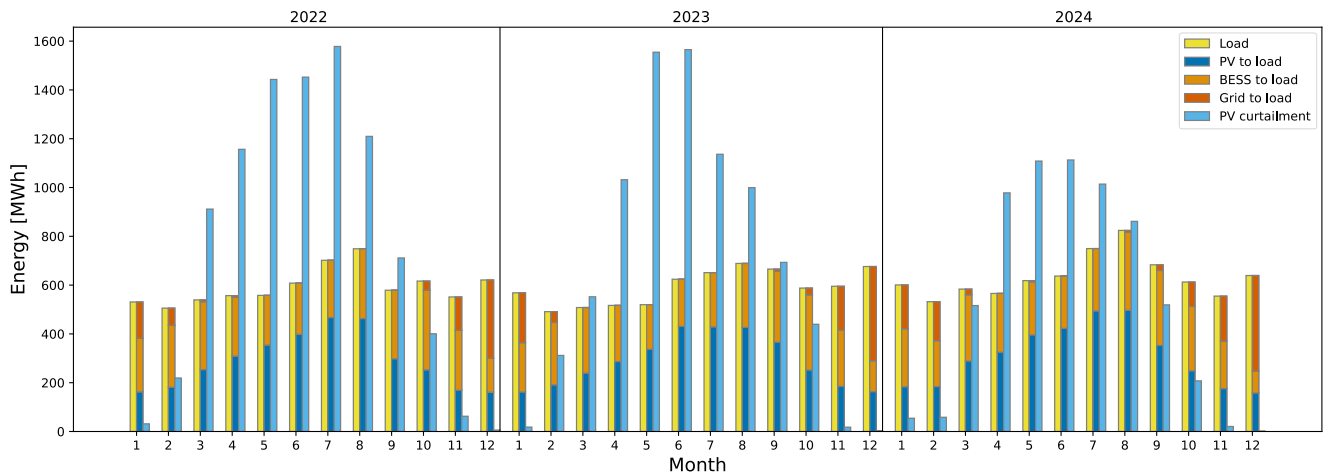
Fig. 5. Monthly load, supply allocation, and PV curtailment for BESS-only configuration
