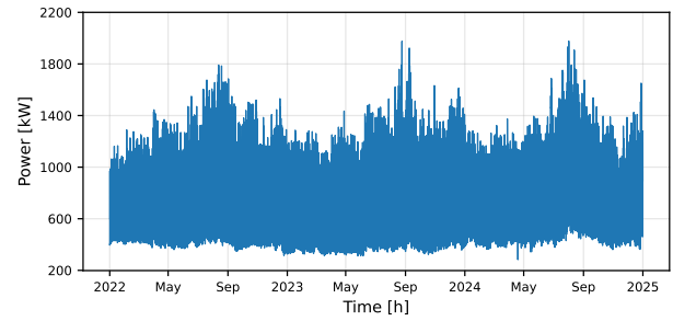
Fig. 2. Hourly load demand profiles of the airport (2022–2024).
