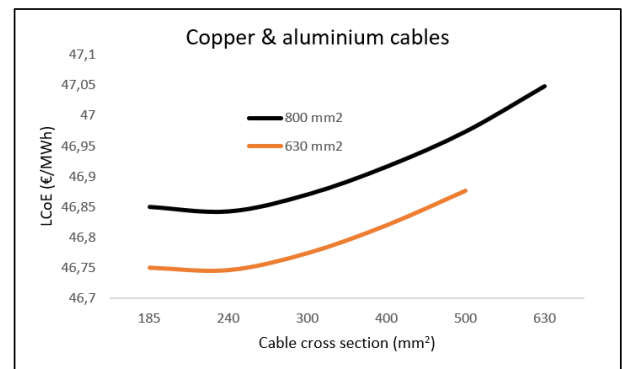
Fig.1.-LCoE vs cable cross section for OWF of 1 GW.
