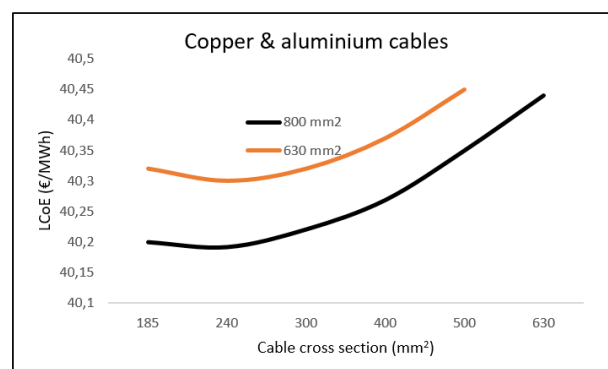
Fig.3-LCoE vs cable cross section for OWF of 1,4 GW.
