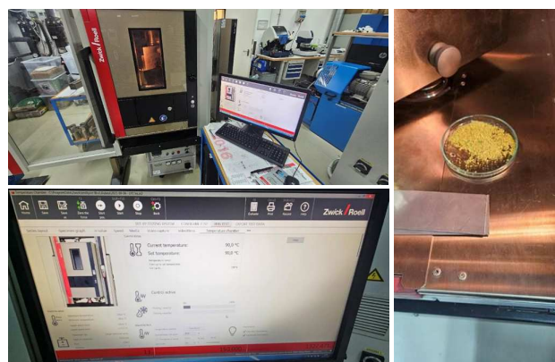
Fig. 2. Thermal treatment of insulation samples in a laboratory temperature chamber, including sample placement, heating environment, and temperature control interface
