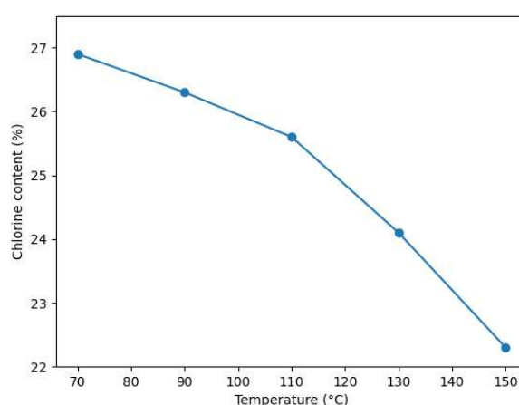
Fig. 7. Variation of chlorine content in PVC insulation as a function of temperature
