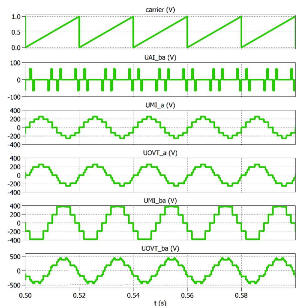
Fig.11 The waveforms of selected voltages obtained for the control strategy described by the vector map shown in Figure 7.
