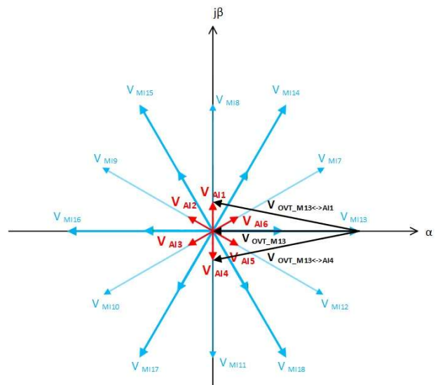
Fig.5. The formation concept of vectors V_{OVTk} – step 1.
