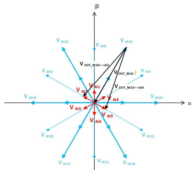
Fig.6. The formation concept of vectors V_{OVTk} – step 2.
