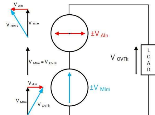
Fig.2. The formation concept of vectors V_{OVTk} .
