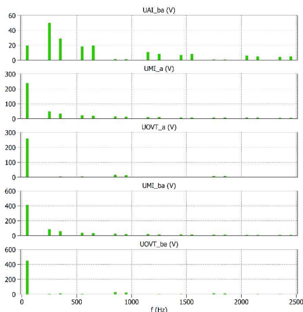
Fig.14. The amplitude spectra of the voltage waveforms from Figure 13.
